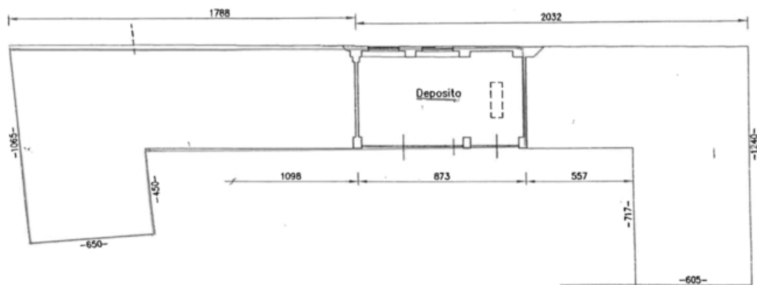
PIANO TERRA h= 302 m
