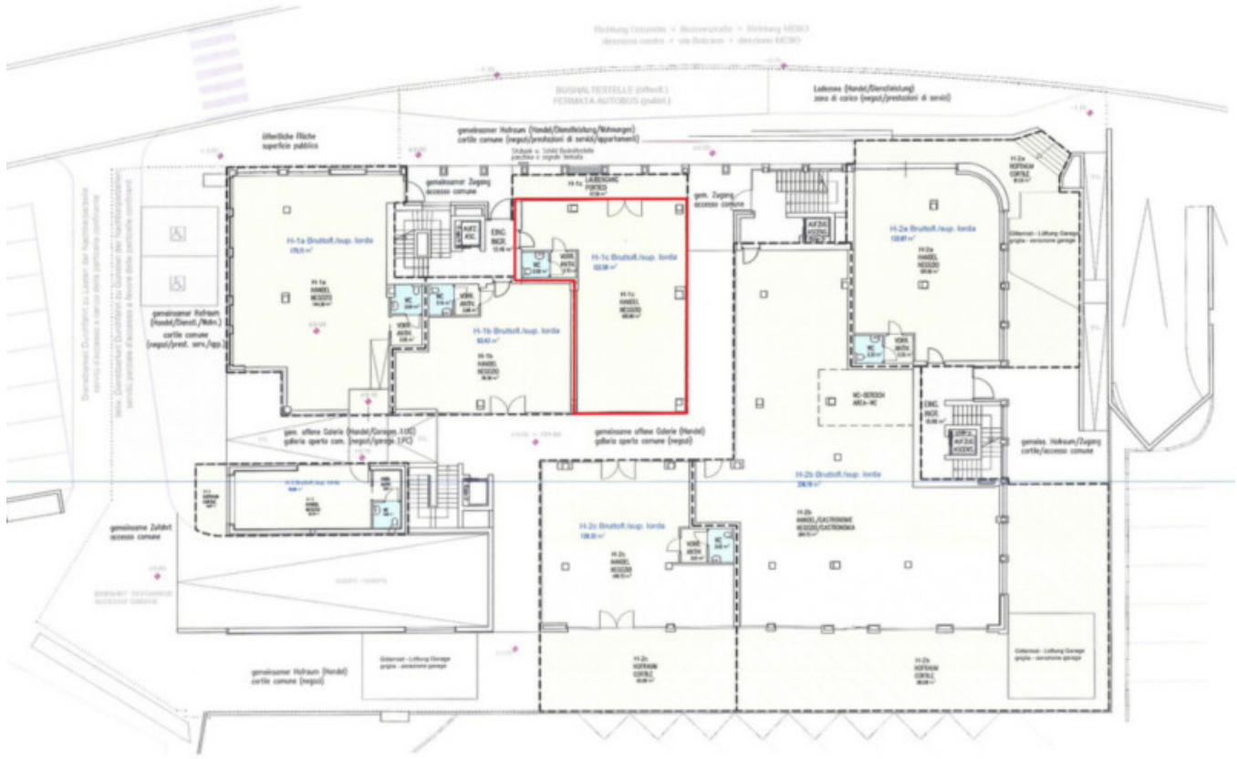
EDGESCHOOS 1:200 PIANO TERRA 1:200
