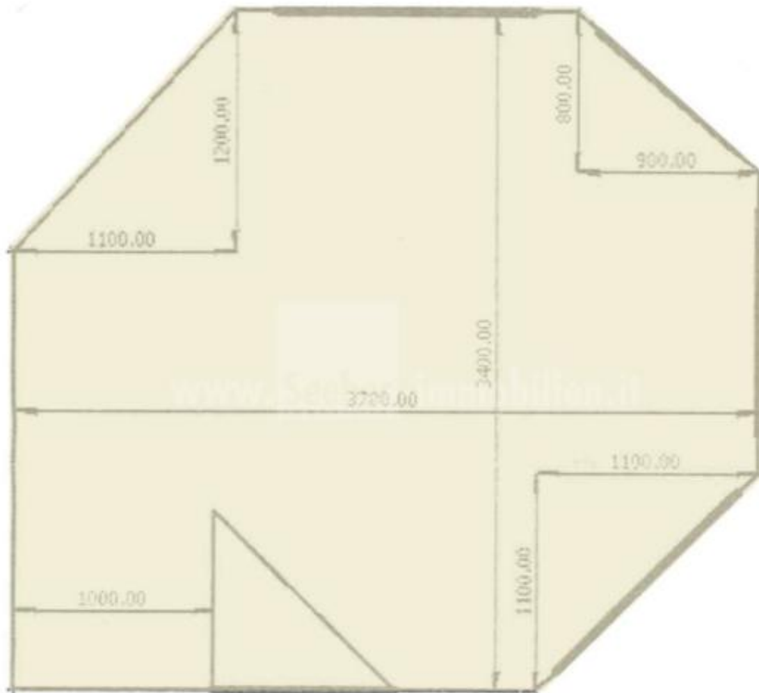
Erdgeschoss-piano terra
