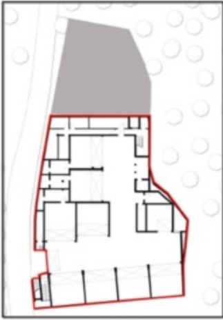
Piano Interrato Ebene -1
