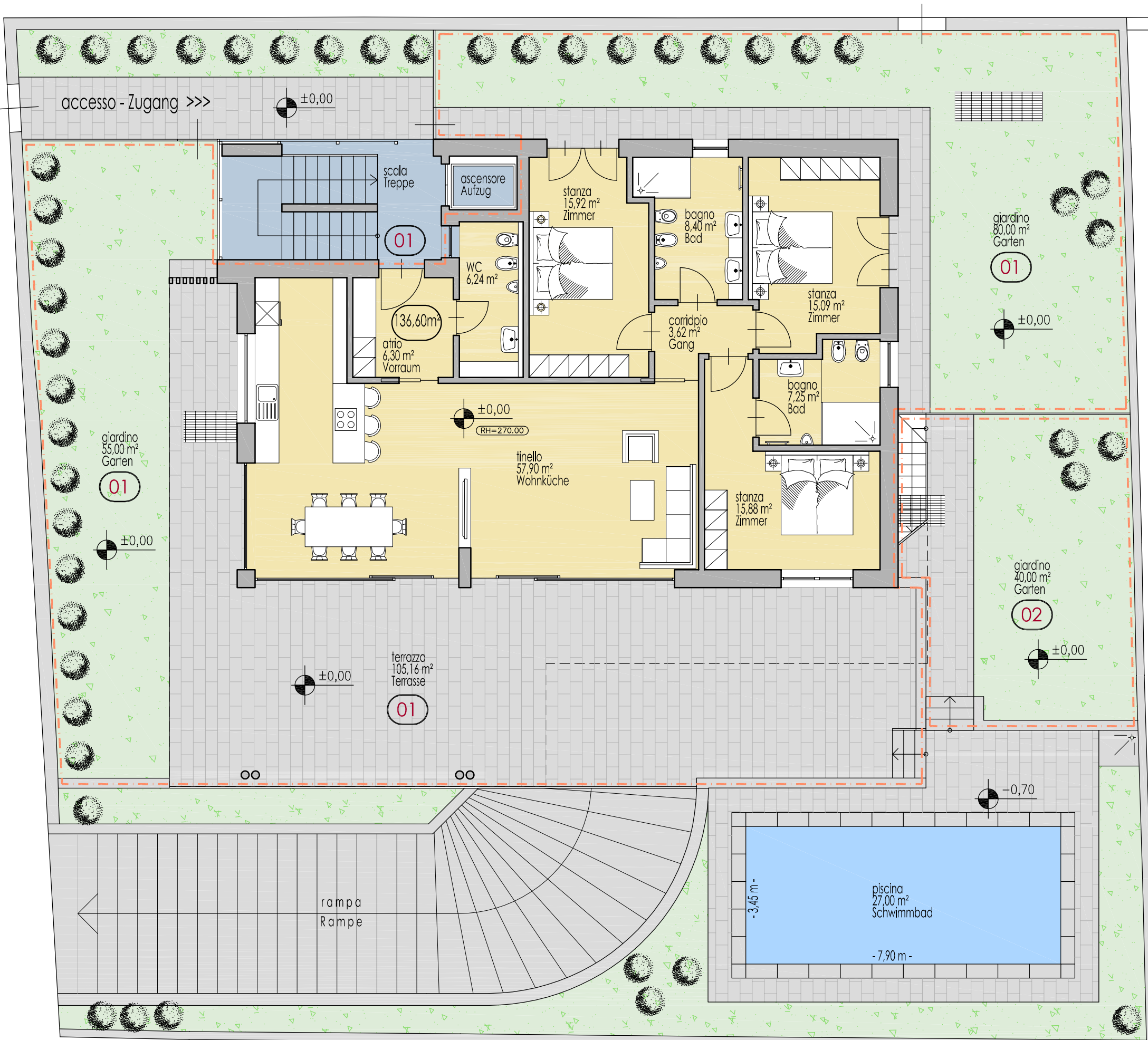
Piano terra - Erdgeschoss
