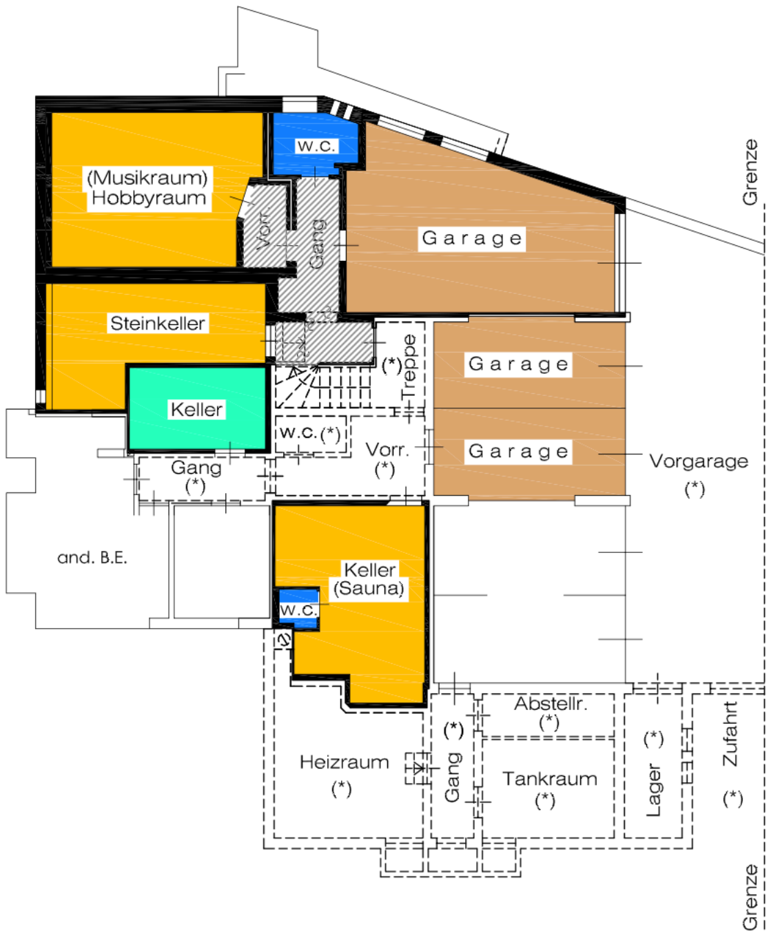
Kellergeschoss - Piano Cantina H=3.00m.
