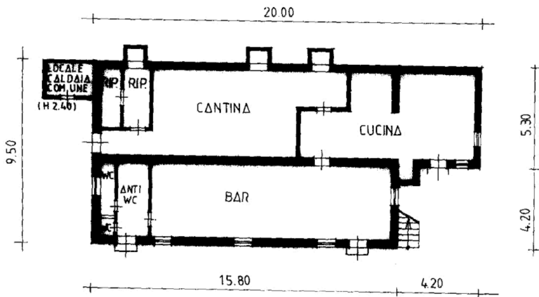
PIANO TERRA h 2.55
